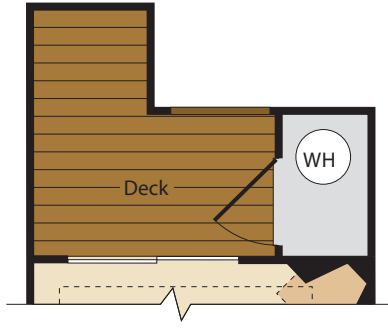
Corner Unit Deck Configuration
